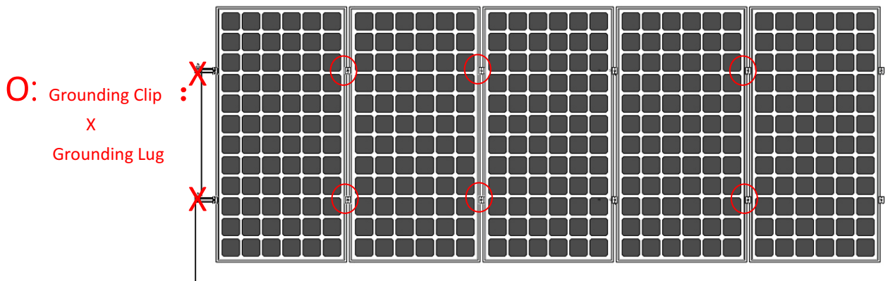
Odd Number of Modules in row
